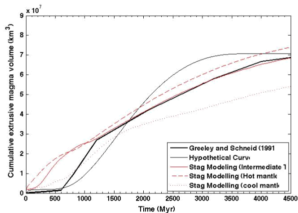
Figure 1: Evolution of the volcanic production on Mars for different models, from observation and numerical modeling. Primordial crust has been excluded from this figure.
