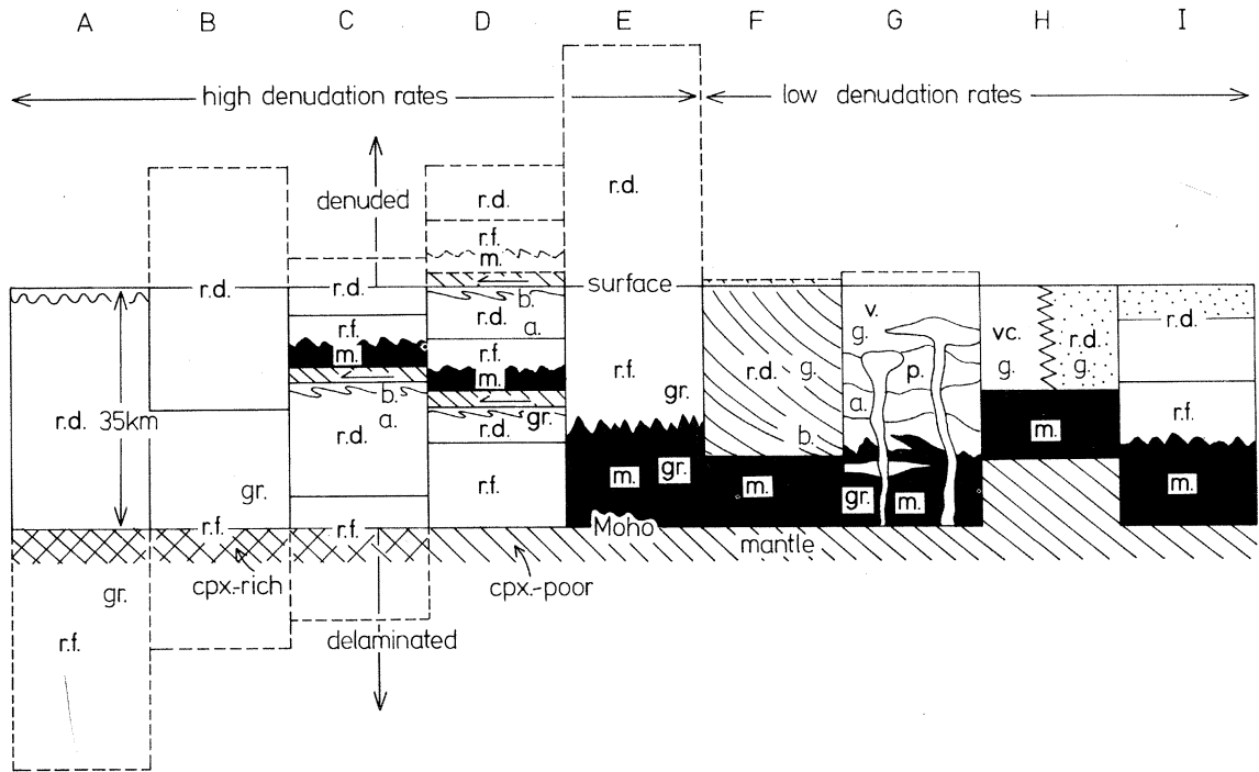
FIGURE 3. Schematic sections of various types of continental crust discussed in the text: A–E, crust thickened by shortening (A, B, E) and thrusting and (C, D) returned to normal thickness by erosion (B–E) and/or delamination (A–C); F, subduction–accretion crust (cf. figure 2c); G, magmatic arc crust, with plutonic (p.) and volcanic (v.) components; H, crust of rear or intra-arc basin with arc-derived volcanoclastic sediment (vc.) and/or continent-derived radiogenic sediment (rd.); I, crust of graben system. Key to shading and abbreviations; solid black shading (m.), mafic lower crust; rd., radiogenic upper crust and sediments; r.f., refractory lower crust; a., amphibolite facies; b., blueschist facies; g., greenschist facies; gr., granulite facies.
